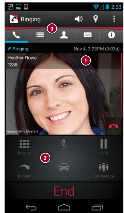
Android smartphone
